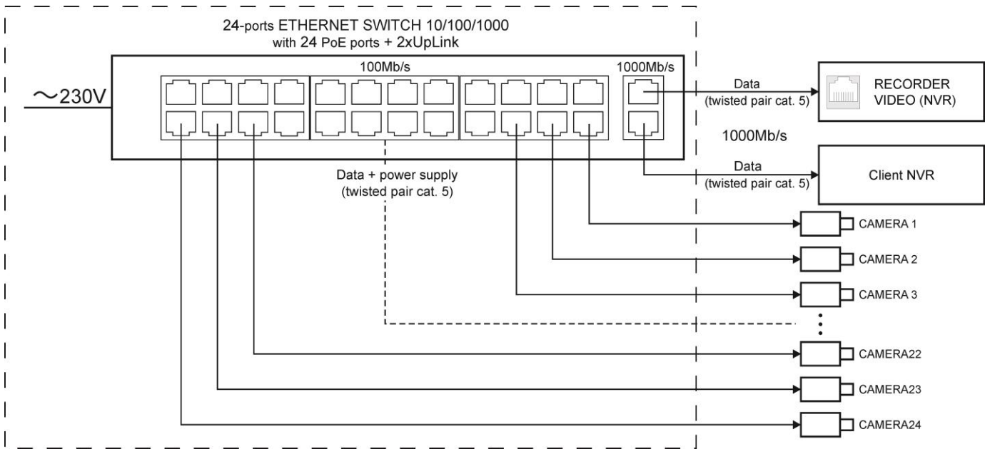
Fig. 1. Block diagram.
